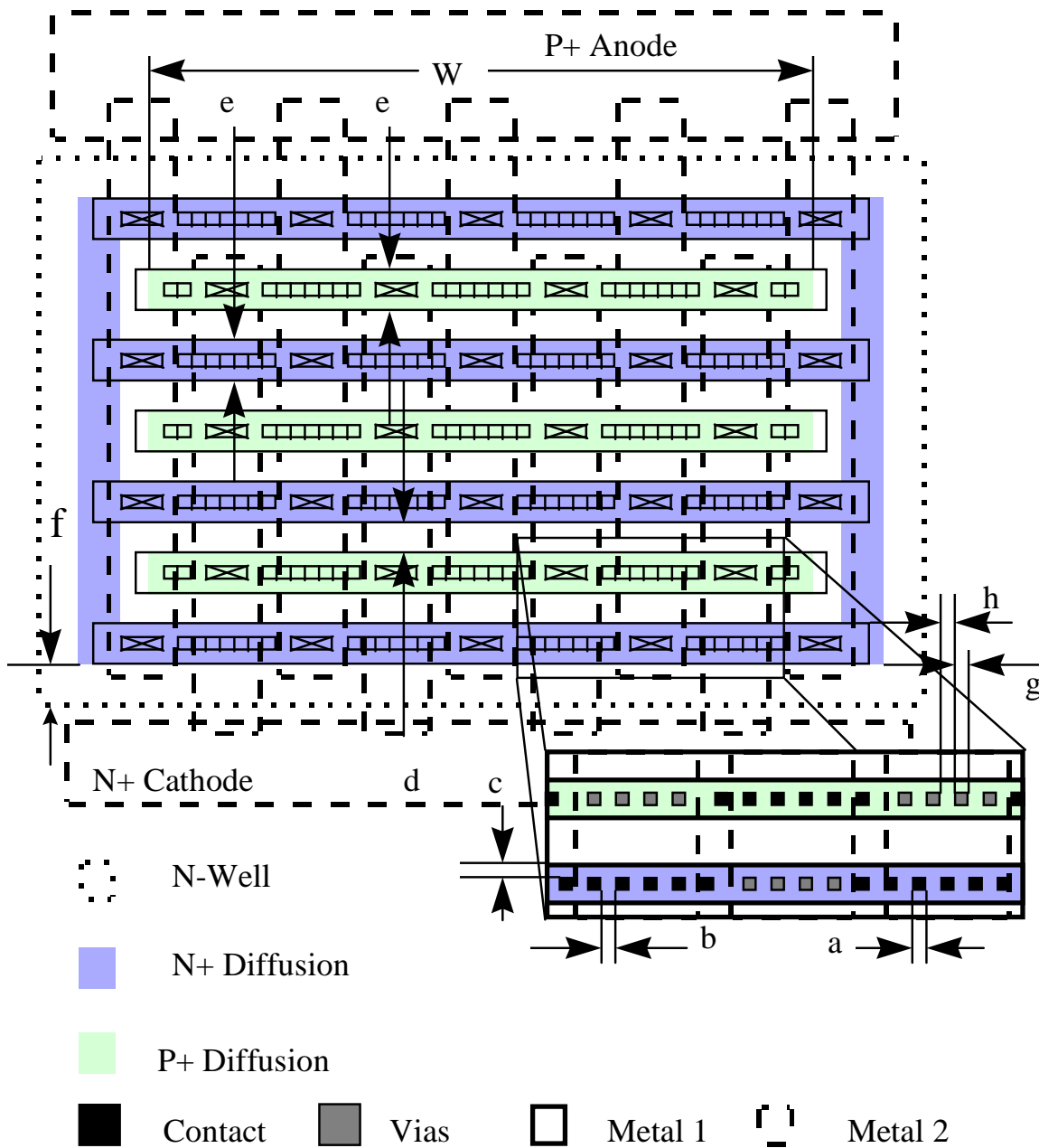
Figure 7 Three-Finger P+ to N-Well Diode
