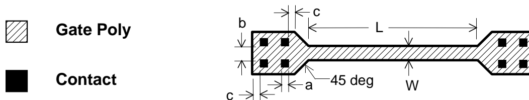
Figure 4 Polysilicon Resistor
