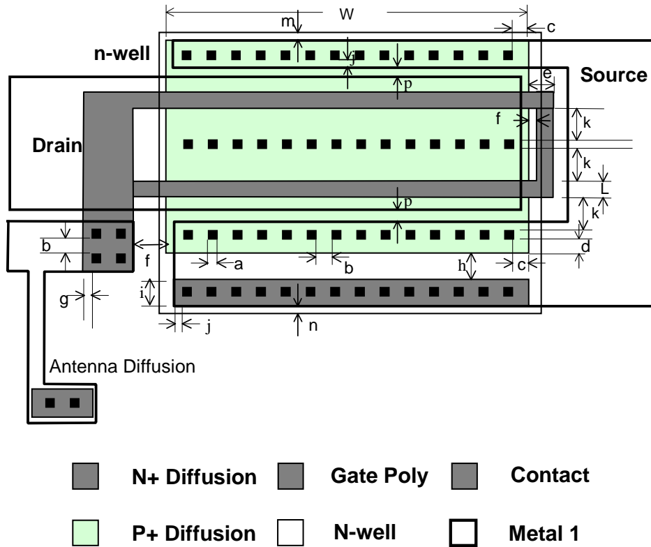
Figure 20 Multi-Finger P-Channel MOSFET
